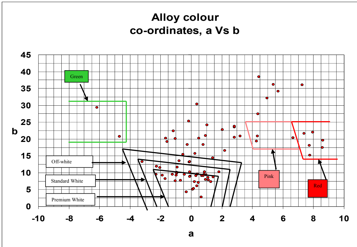
Figure 4: CIELab co-ordinates, a Vs b, data plotted for all samples. Boxes are potential grades (colour boxes) for all standard colour gold alloys
